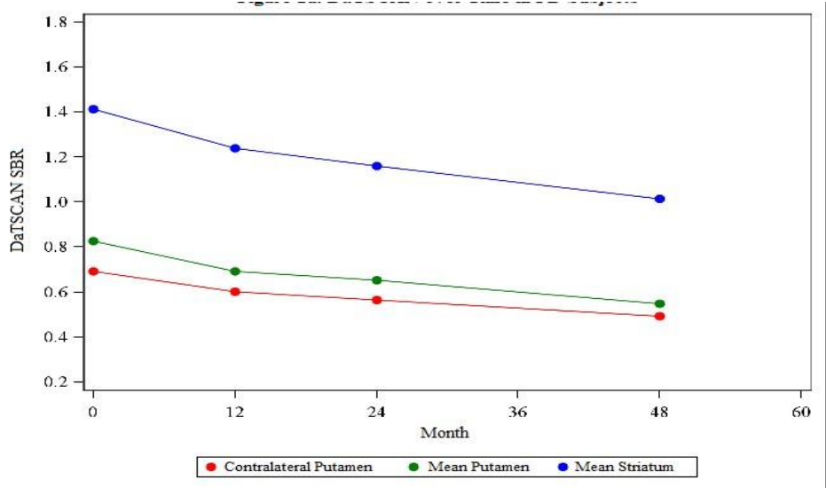
Figure 2 Change in DAT SBR in PPMI PD participants
